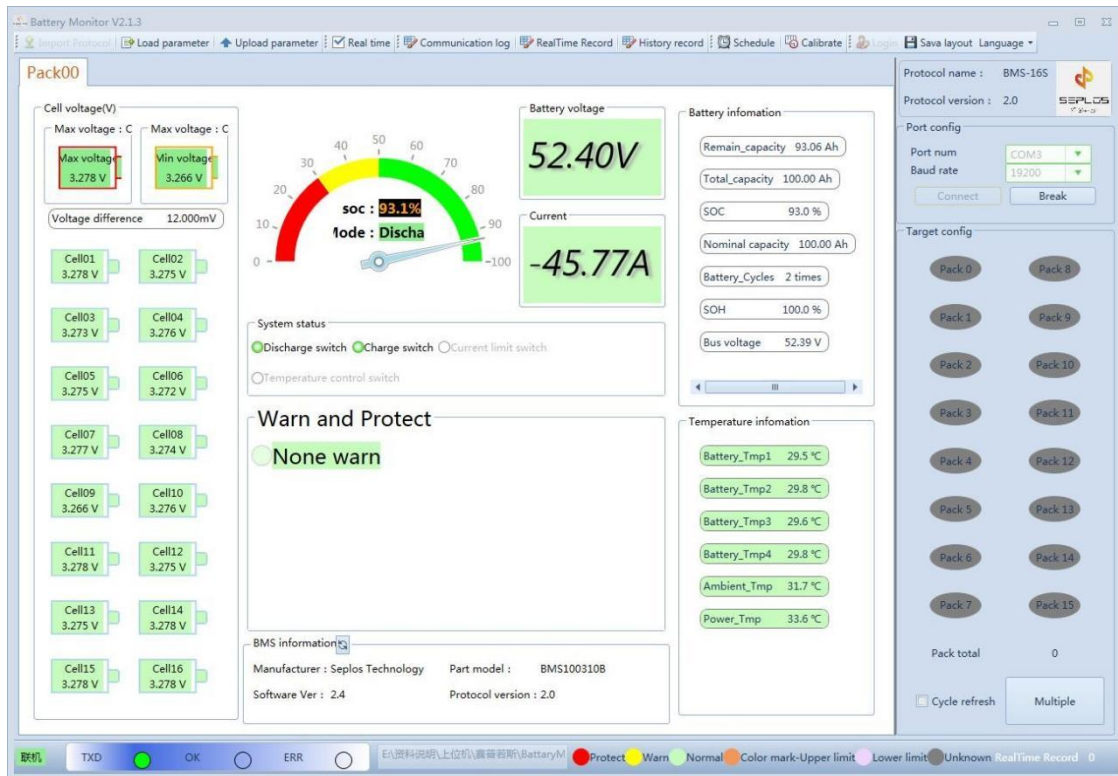
Software interface
